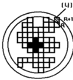
FIG. 1. The model of random successive growth on a square lattice with a seed of five neighboring sites, where R is the maximum radius if the cluster composed of filled and open squares and (i,j) is the potential growth site.
